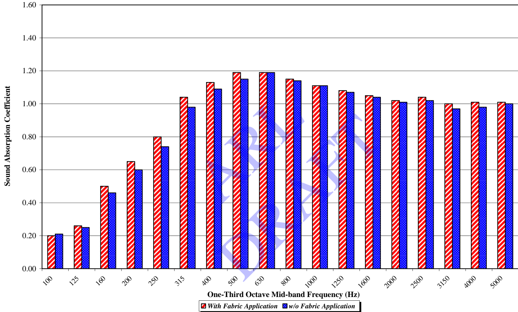
Carnegie Johns Manville Equipment Spin-Glas® Board WITH (ARL-SA6715) and WITHOUT (ARL-SA6712) 6207 PIPELINE (100% XOREL), Unbacked, Thickness 2" - Type A Mounting
